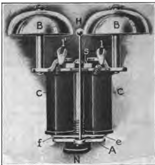
FIG. 75.—Telephone ringer.
